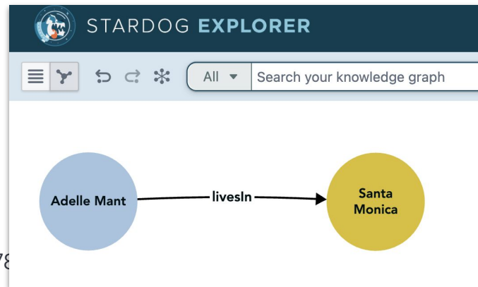
Human-friendly visualisation uses Labels
